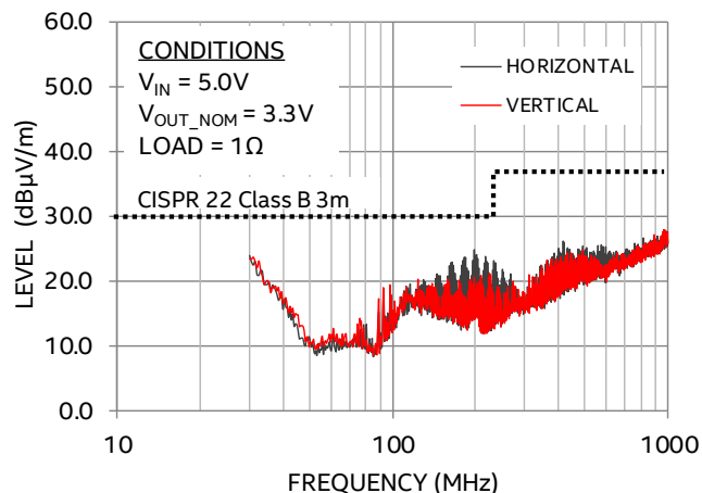
EMI Performance
