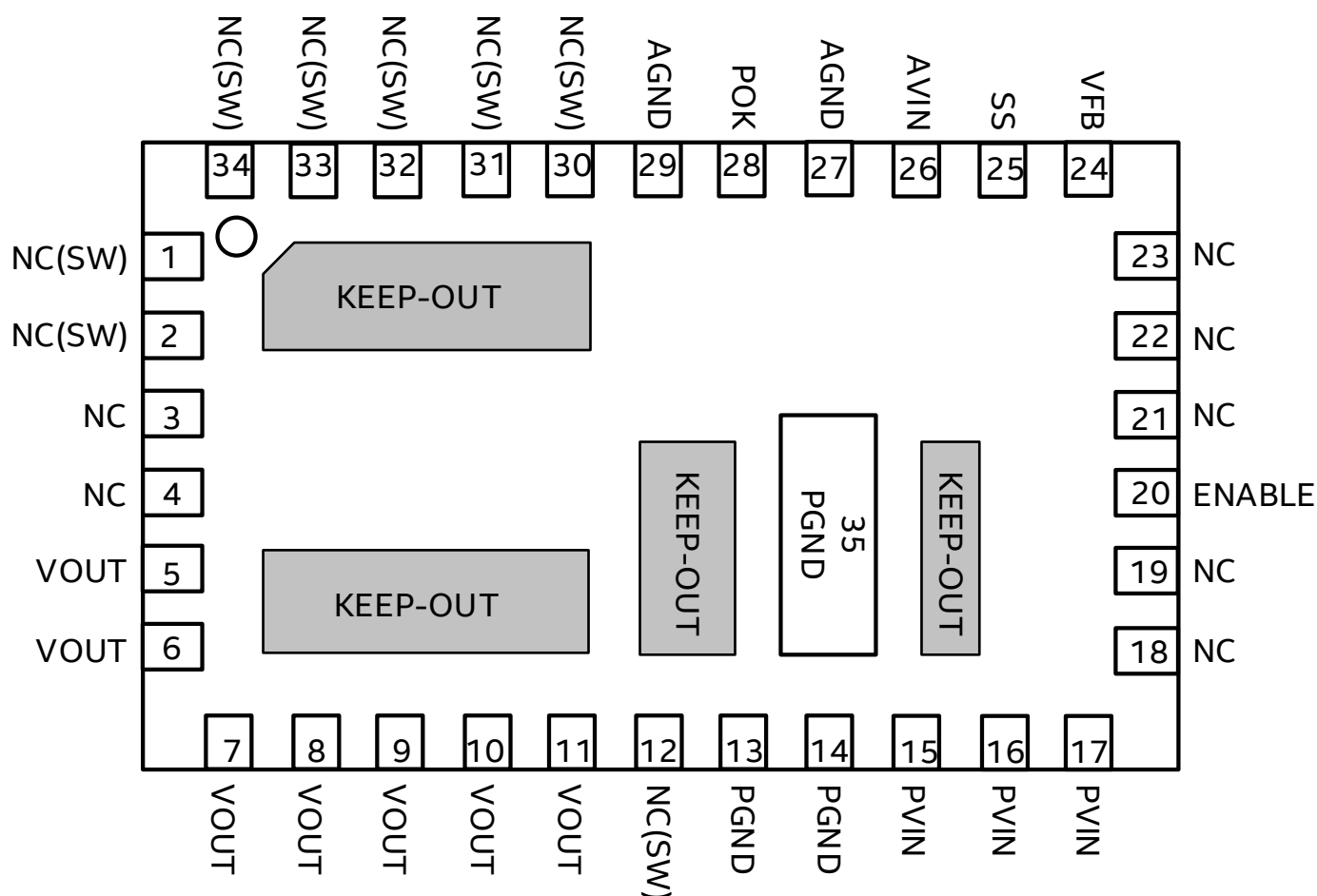
Figure 3: Pin Diagram (Top View)
