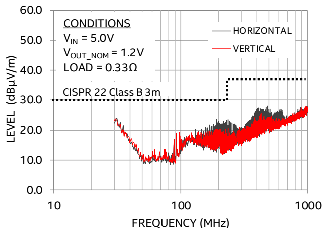
EMI Performance
